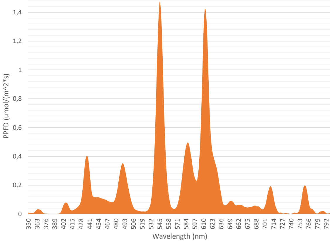
Reach-in Fluorescent tubes_RI102 (Weiss-Gallenkamp reach-in growth chamber)
