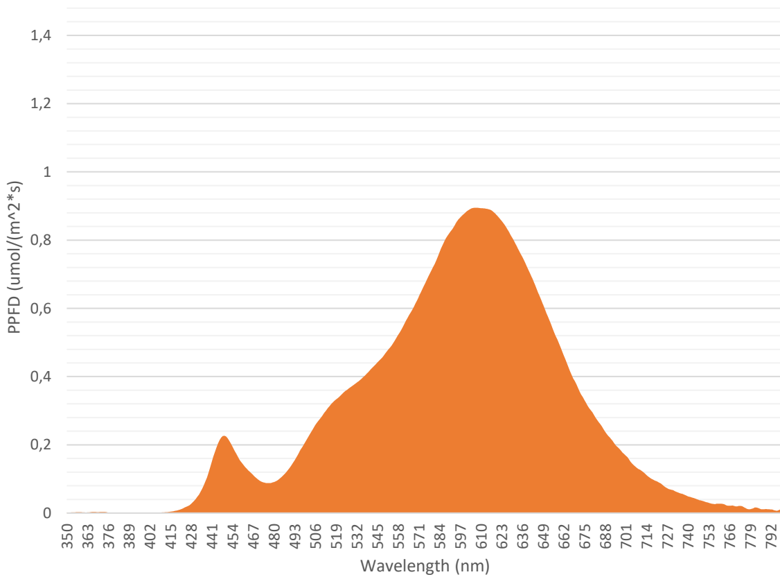
Warm White LED_PSI Walk-in chamber 1
