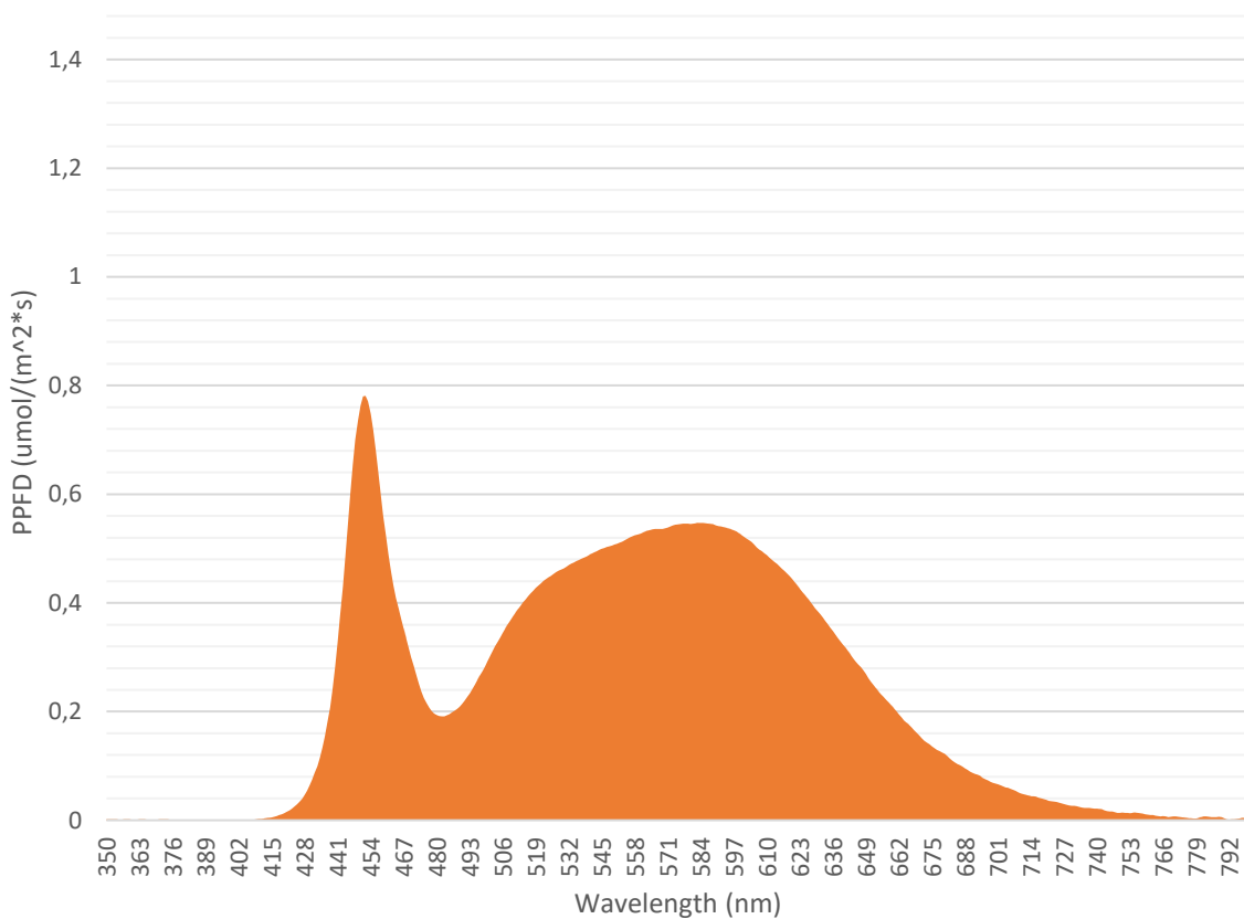
Cool white LED_RI109 (PSI FS-RR 1600 Reach-in growth chamber)
