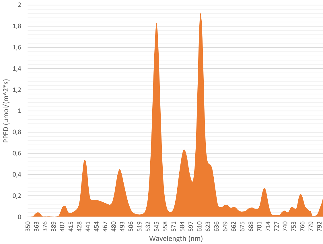
Fluorescent light tubes_Cultivation room 555
